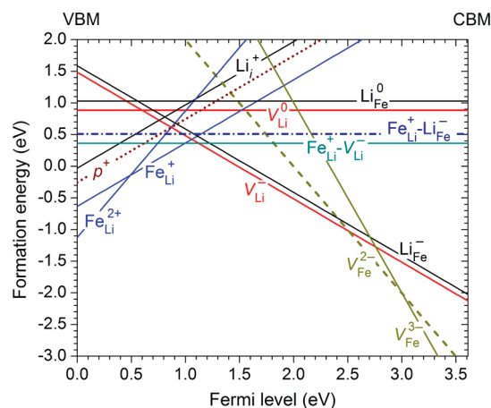
Figure 3. Calculated formation energies of native point defects and defect complexes in LiFePO 4 , plotted as a function of Fermi level with respect to the VBM. The energies are obtained at point A in the chemical-potential diagram for \mu_{\text{O}_2} = -4.59 eV (cf., Figure 1), representing equilibrium with Fe 2 O 3 and Fe 3 (PO 4 ) 2 .
