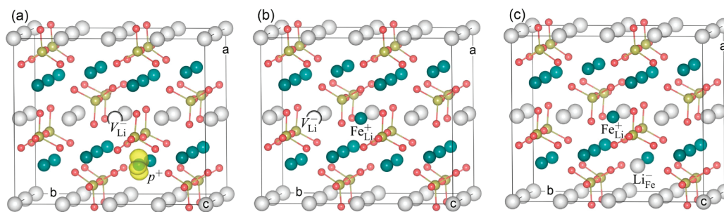
Figure 4. Defects in LiFePO 4 : (a) V_{\text{Li}}^0 can be regarded as a complex of V_{\text{Li}}^- (represented by the empty sphere) and hole polaron p^+ (i.e., \text{Fe}^{3+} ; decorated with the square of the wave functions of the lowest unoccupied state in the electronic structure of LiFePO 4 in the presence of V_{\text{Li}}^0 ); (b) \text{Fe}_{\text{Li}}^+ - V_{\text{Li}}^- , a complex of \text{Fe}_{\text{Li}}^+ and V_{\text{Li}}^- ; and (c) \text{Fe}_{\text{Li}}^+ - \text{Li}_{\text{Fe}}^- , a complex of \text{Fe}_{\text{Li}}^+ and \text{Li}_{\text{Fe}}^- . Large (gray) spheres are Li, medium (blue) spheres are Fe, small (yellow) spheres are P, and smaller (red) spheres are O.
