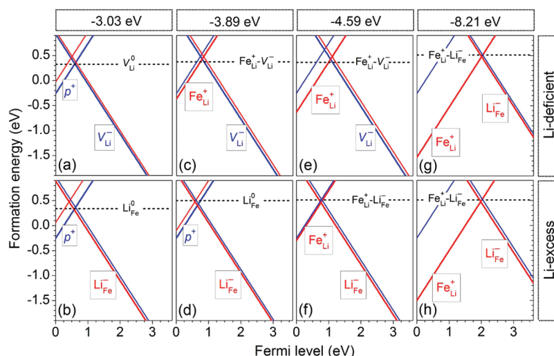
Figure 7. Calculated formation energies of the low-energy positively and negatively charged point defects (i.e., p^+ , \text{Fe}_{\text{Li}}^+ , \text{V}_{\text{Li}}^- , and \text{Li}_{\text{Fe}}^- ) and their neutral defect complexes, plotted as a function of Fermi level with respect to the VBM, under different conditions: \mu_{\text{O}_2} = -3.03, -3.89, -4.59 , and -8.21 eV, and Li-deficient and Li-excess environments. Panels (a)–(h) correspond to conditions (1)–(8); see text. Only the complex that consists of the lowest-energy negatively and positively charged point defects is included.
