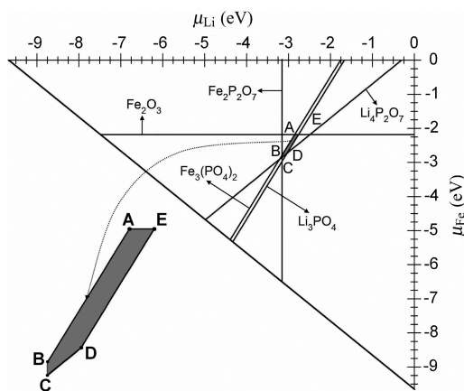
Figure 1. Chemical-potential diagram for \text{LiFePO}_4 at \mu_{\text{O}_2} = -4.59 eV. The \mu_{\text{O}_2} axis extends out of the page. Only phases that can be in equilibrium with \text{LiFePO}_4 are included, and the lines delineating these phases define the stability region of \text{LiFePO}_4 , here shown as a shaded polygon.
