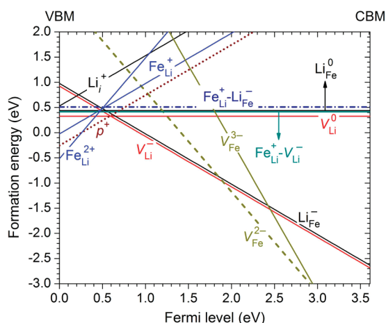
Figure 5. Calculated formation energies of native point defects and defect complexes in LiFePO 4 , plotted as a function of Fermi level with respect to the VBM. The energies are obtained at \mu_{\text{O}_2} = -3.03 eV, and equilibrium with Fe 2 O 3 and Fe 7 (PO 4 ) 6 is assumed.
