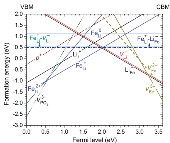
Figure 6. Calculated formation energies of native point defects and defect complexes in LiFePO 4 , plotted as a function of Fermi level with respect to the VBM. The energies are obtained at \mu_{\text{O}_2} = -8.21 eV, and equilibrium with Fe 2 P and Fe 3 P is assumed.
